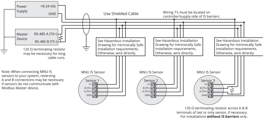
Modbus System Wiring
