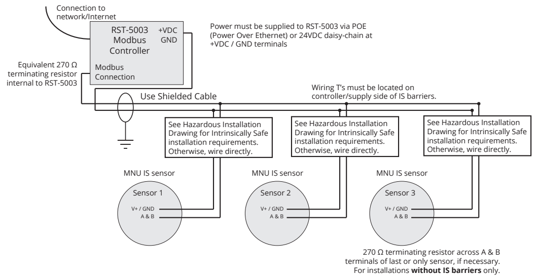
Modbus System Wiring with RST-5003 and Power Over Ethernet (POE) or VDC
