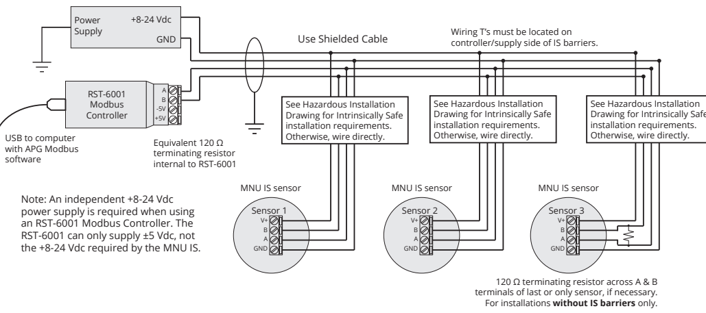
Modbus System Wiring with RST-6001
