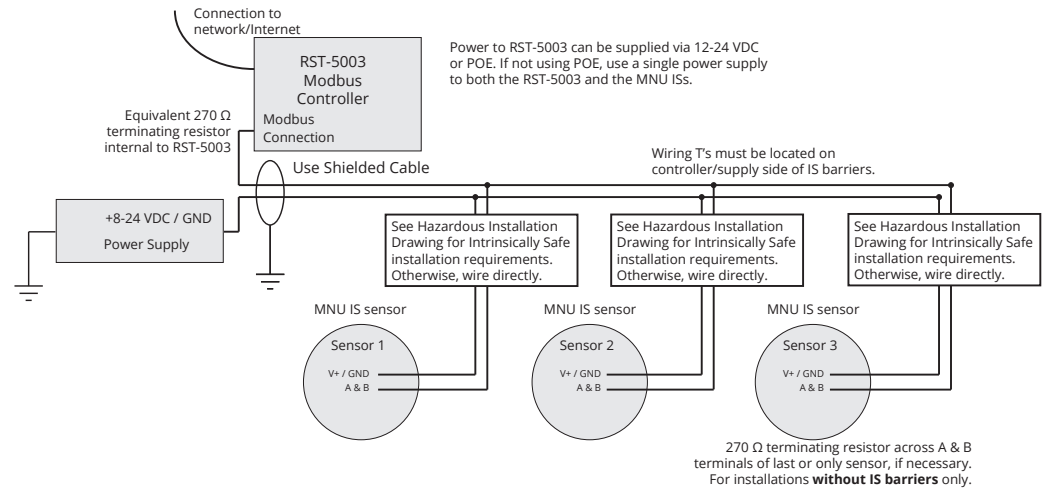
Modbus System Wiring with RST-5003 and Independent Power Supply
